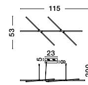
RACCIO - 9695213 Triac Dimmable Black Metal & Acrylic LED 27 Watt 230 Volt 1308Lm 3000K IP20 L: 115 W: 53 H: 200 cm
