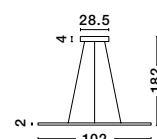
ODERICK - 9100145 Sandy Black Aluminium & Acrylic LED 44 Watt 230 Volt 1346Lm 3000K IP20 D: 102 H: 182 cm
