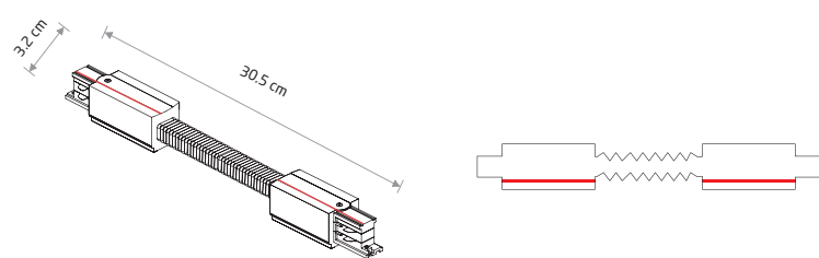
15 CTLS POWER FLEX CONNECTOR plastic, copper 8698 8700
